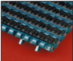
1005 SUPERGRIP BELT WITH DOUBLE POSITRACK ON ONE SIDE OF THE BELT
