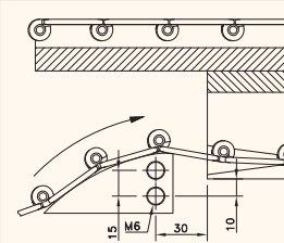
RETURN GUIDE SHOE
