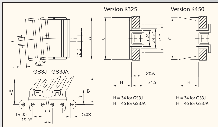
SNAP-ON 3-FINGER GRIPPER ¾" PITCH PLASTIC TAB
