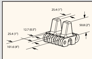
T2 DIMENSIONS
