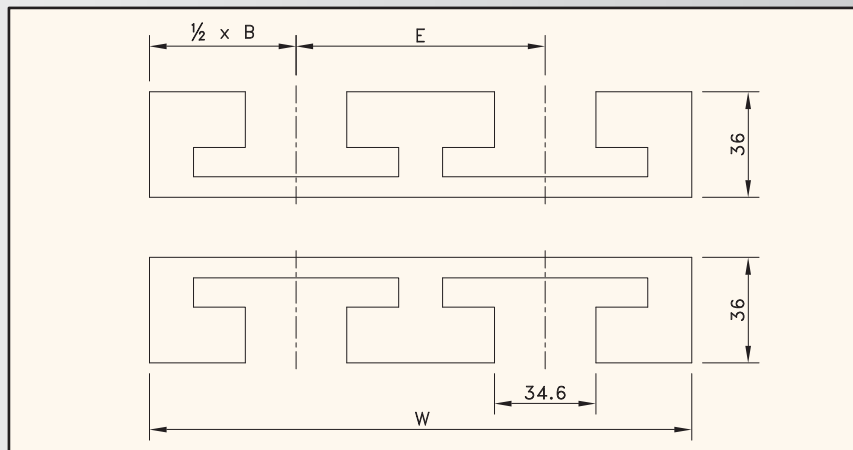
KTU 300 FOR PLATE TOP CHAINS
