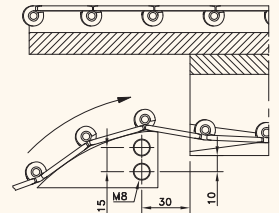
RETURN GUIDE SHOE
