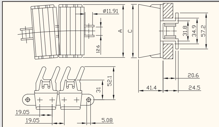
SNAP-ON 2-FINGER GRIPPER ¾" PITCH PLASTIC TAB
